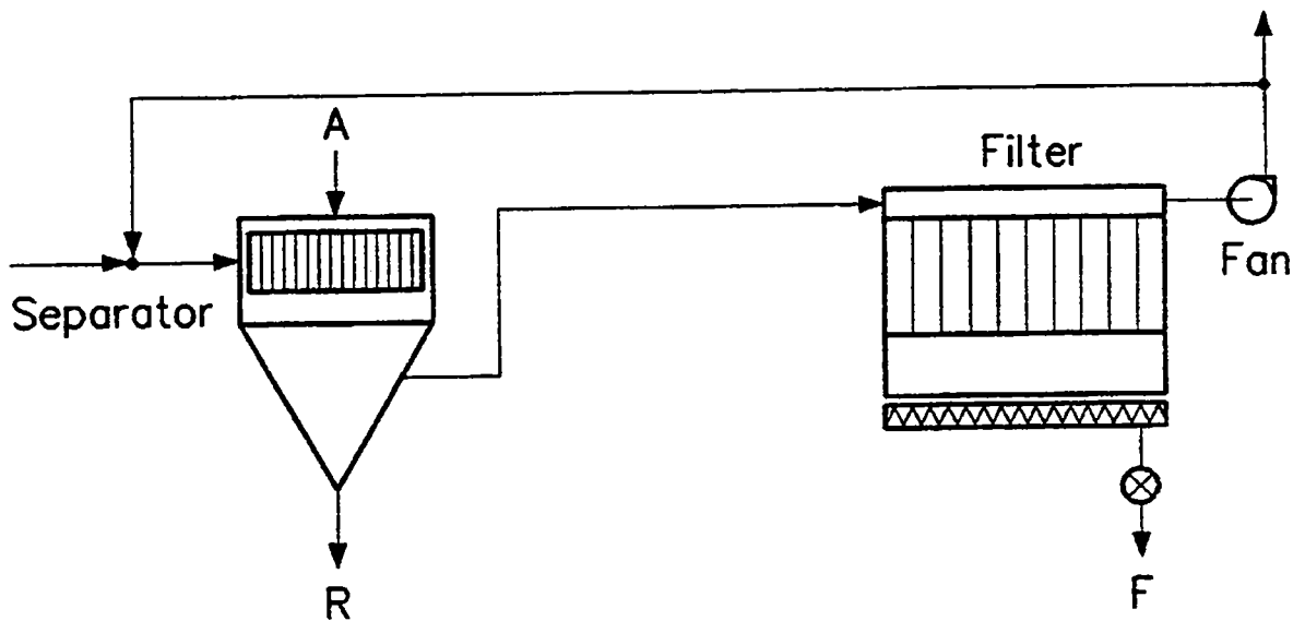
Figure 3 Single Pass Separator (Rotor Type)
